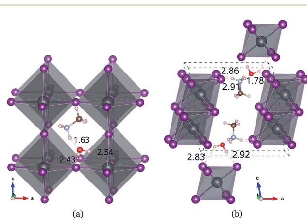
Fig. 1 Polyhedral view of water intercalated phase MAPbI 3 ·H 2 O (a) and monohydrated phase MAPbI 3 ·H 2 O (b). Hydrogen bonds are marked with dotted lines and the bond lengths are presented in units of angstrom (dark grey: Pb; purple: I; brown: C; light blue: N; red: O; light pink: H).
