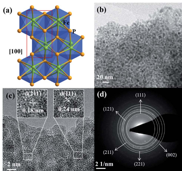
Fig. 6 (a) The crystal structure of \text{FeP} crystallizing in the orthorhombic space group \text{Pna}2_1 (shown along [100] ; the unit cell is shown in red). (b) TEM image displaying homogeneously distributed nanoparticles of 2–5 nm in size. (c), HR-TEM image with d -spacing of 0.18 and 0.24 nm (in the inset) corresponding to (211) and (111) planes. (d) SAED pattern exhibiting characteristic rings confirming the phase-purity of \text{FeP} (JCPDS 71-2262).
