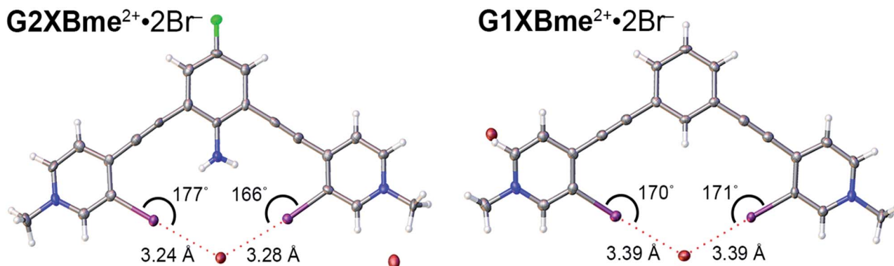
Fig. 5 Bidentate XBing conformations of \text{G2XBme}^{2+} \cdot 2\text{Br}^- (left) and \text{G1XBme}^{2+} \cdot 2\text{Br}^- (right). XB distances and angles are displayed. Thermal ellipsoids are drawn at the 50% probability level. \text{G1XBme}^{2+} \cdot 2\text{Br}^- crystallized with a methanol molecule which HBs with noncoordinating \text{Br}^- and is omitted for clarity.
