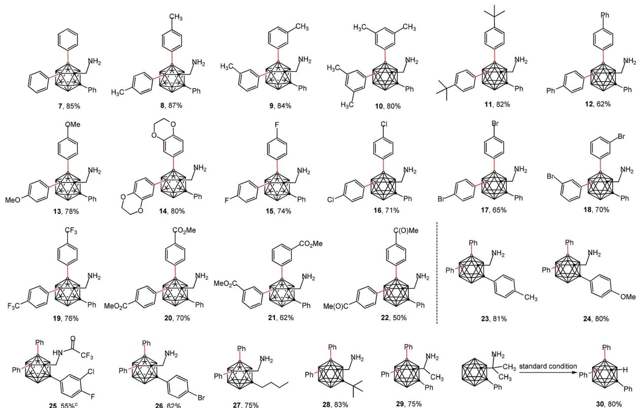
Scope of aryl iodides (7-22) and o-carboranyl methylamines (23-30)
