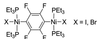
Scheme 4 Dinuclear product [\text{trans-NiX}(\text{PEt}_3)_2]_2(\mu\text{-}2,3,5,6\text{-C}_6\text{F}_4) .
