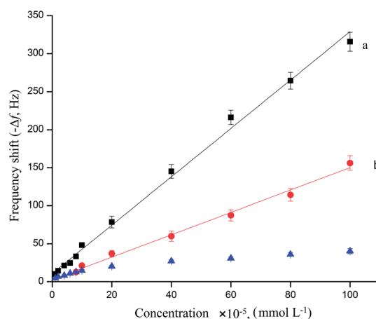
Fig. 5 Calibration curves of the MIP/rGO-AuPs/AuE (a), MIP/AuNPs/AuE (b), and NIP/rGO-AuPs/AuE (c) to AM.
