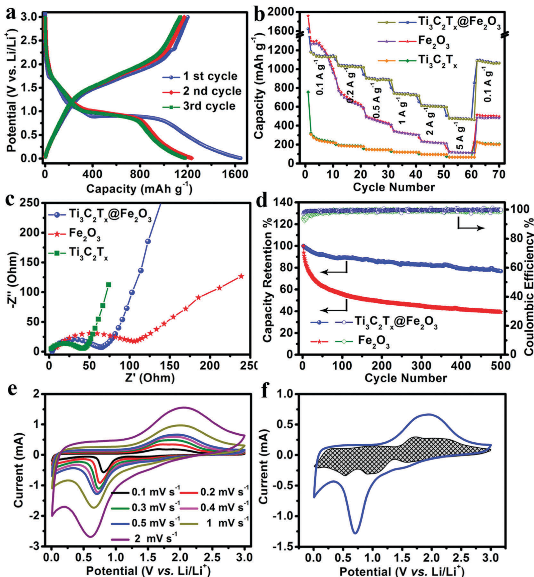
Fig. 3 Lithium storage performance of the Fe_2O_3 , Ti_3C_2T_x and Ti_3C_2T_x@Fe_2O_3 electrodes: (a) the first three charge–discharge cycles of the Ti_3C_2T_x@Fe_2O_3 hybrid electrode at a current density of 0.1 \text{ A g}^{-1} . (b) Rate performances and (c) EIS of the Fe_2O_3 , Ti_3C_2T_x and Ti_3C_2T_x@Fe_2O_3 electrodes. (d) Cycling stability of the Fe_2O_3 and Ti_3C_2T_x@Fe_2O_3 electrodes at a current density of 5 \text{ A g}^{-1} . (e) CV curves of a Ti_3C_2T_x@Fe_2O_3 electrode at different scan rates. (f) The capacity separation of the Ti_3C_2T_x@Fe_2O_3 hybrid electrode at a scan rate of 0.5 \text{ mV s}^{-1} .
