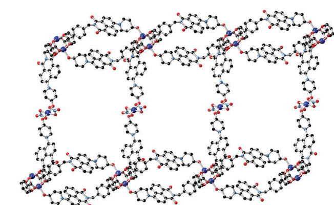
Fig. 6 (top) The two distinct copper coordination environments within the structure of 4 , with labelling scheme for coordinating heteroatoms. (bottom) Extended structure of a single layer of 4 , consisting of linear bridges between looped L2 -paddlewheel chains. Hydrogen atoms and backbone disorder are omitted for clarity. Symmetry codes used to generate equivalent atoms: (i) 1/2 - x, 3/2 - y, 1 - z ; (ii) 2 - x, 1 - y, 2 - z .
