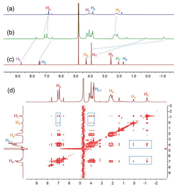
Fig. 1 ^1\text{H} NMR spectra (400 MHz, \text{D}_2\text{O} , 298 K): (a) WP5-P (10.0 mM); (b) WP5-P (10.0 mM) and G1 (10.0 mM); (c) G1 (10.0 mM). (d) 2D NOESY spectrum of a mixture of WP5-P (10.0 mM) and G1 (10.0 mM). The NOE correlation signals that confirm the host-guest interactions are marked on the spectrum.
