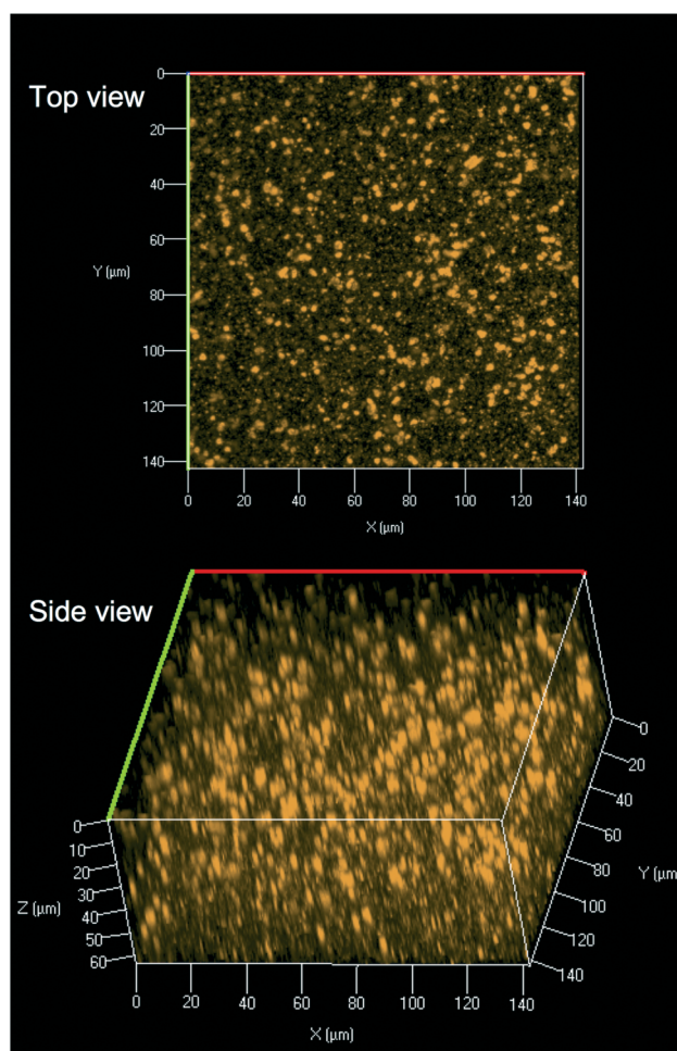
Fig. 2 142.86 \mu\text{m} \times 142.86\text{ }\mu\text{m} CLSM 64 \mu\text{m} Z-stack image of CdSe/ZnS-PMMA polymer nanocomposite obtained with 458 nm excitation. Any emission detected above a 505 nm cut-off filter is shown in orange, which includes the QD \lambda_{\text{max}} = 594\text{ nm} .
