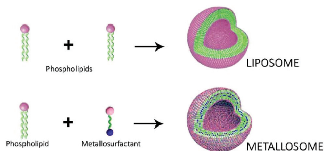
Scheme 2 Formation of liposomes with phospholipids or metallosomes by mixing metallocsurfactants and phospholipids.
