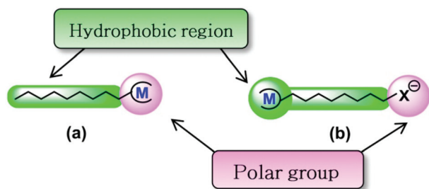
Scheme 1 Representation of metallocsurfactants with the metal (M) in the polar head group (a) or in the hydrophobic region (b).
