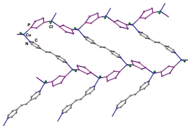
Fig. 2 Fragment of a single layer in the neutral 2D polymeric network 4: \text{Cp}^*\text{FeP}_5 are represented as cyclo- \text{P}_5 fragments; H atoms are omitted for clarity.
