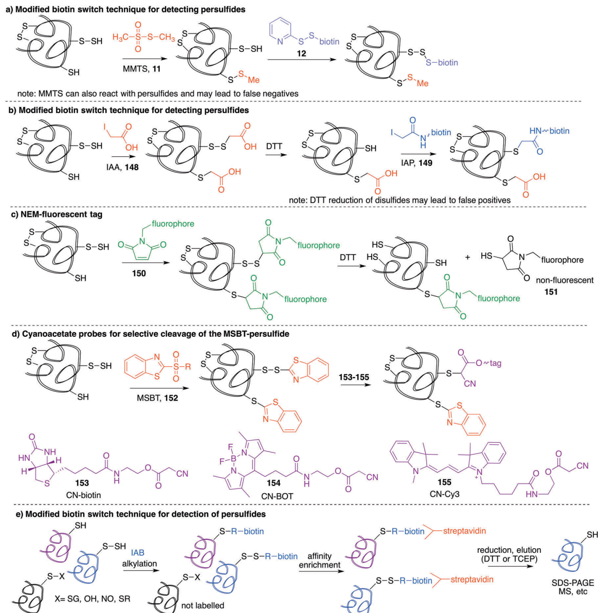
Fig. 17 (a and b) A modified biotin switch technique for detecting cysteine persulfides. Note that in the initial blocking step, MMTS ( 11 ) may also react with the cysteine persulfide. Iodoacetic acid (IAA, 148 ) is a more suitable blocking reagent because both thiols and persulfides are alkylated and the latter can be reduced and selectively labelled with biotin. (c) A fluorescent maleimide ( 150 ) can react with cysteine thiols and persulfides. Cleaving the disulfide product derived from the persulfide results in a decrease in fluorescence that can be monitored. (d) Reagent 152 reacts with cysteine thiols and persulfides. The disulfide formed from the reaction of cysteine persulfide and 152 can subsequently be tagged by reaction to a nucleophilic cyanoacetate group conjugated to biotin or a fluorescent tag. (e) A variation of the biotin switch technique illustrating how cysteine persulfides can be enriched by binding to immobilised streptavidin. The proteins bound through the persulfide (but not through the non-reducible thioether) can then be cleaved with DTT or TCEP and isolated for analysis.
