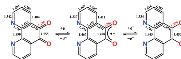
Scheme 1 Three-membered electron transfer series for pd showing calculated bond distances.
