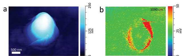
Fig. 4 (a) 3D height image of a glucose/NaCl (1 : 1 mass ratio) particle with a volume equivalent diameter of 510 nm (b) chemical map of the glucose rich regions of the particle taken at 1090\text{ cm}^{-1} .
