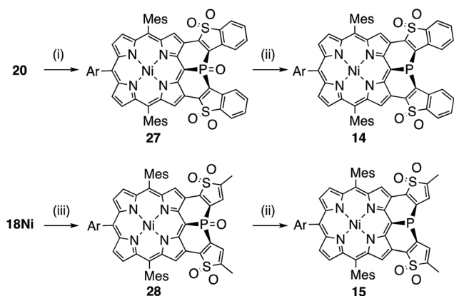
Scheme 3 Synthesis of (thiophene 1,1-dioxide)-fused porphyrins 14 and 15 (Ar = 3,5-di- tert -butylphenyl). (i) \text{H}_2\text{O}_2 , \text{Na}_2\text{WO}_4 \cdot 2\text{H}_2\text{O} , MeN( n - \text{C}_8\text{H}_{17} ) _3 · \text{HSO}_4 , PhPO(OH) _2 , toluene/ \text{H}_2\text{O} , 50 °C, 84%; (ii) \text{HSiCl}_3 , toluene, 110 °C, ( 14 : 26%, 15 : 28%); (iii) \text{H}_2\text{O}_2 , \text{Na}_2\text{WO}_4 \cdot 2\text{H}_2\text{O} , MeN( n - \text{C}_8\text{H}_{17} ) _3 · \text{HSO}_4 , PhPO(OH) _2 , toluene/ \text{H}_2\text{O} , 70 °C, 43%.
