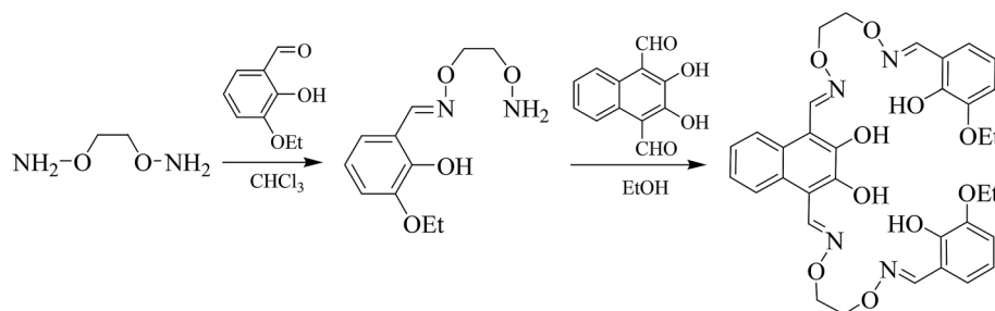
Scheme 1 Synthetic route to bis(salamo)-type tetraoxime ligand H_4L .
