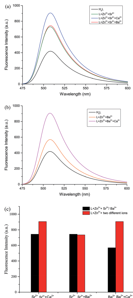
Fig. 6 (a) Fluorescence spectra of complex 2 solution ( 1.0 \times 10^{-5} mol L ^{-1} ) in the absence and presence of various metal ions (1.0 equiv. of Ca(II) and Ba(II)). (b) Fluorescence spectra of complex 3 solution ( 1.0 \times 10^{-5} mol L ^{-1} ) in the absence and presence of various metal ions (1.0 equiv. of Ca(II)). (c) Fluorescence response of L-Zn(II) solution ( 1.0 \times 10^{-5} mol L ^{-1} ) to various metal ions. ex = 367 nm, em = 508 nm.
