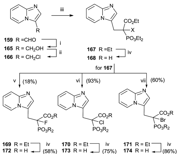
Scheme 30 Reagents and conditions: (i) \text{NaBH}_4 , MeOH, reflux. (ii) \text{SOCl}_2 , reflux, (iii) triethyl phosphonoacetate, NaH, DMF, THF, 0 °C to rt. (iv) 12 M HCl, reflux. (v) Selectfluor, NaH, THF. (vi) N -Chlorosuccinimide, NaH, THF. (vii) N -Bromosuccinimide, NaH, THF.
