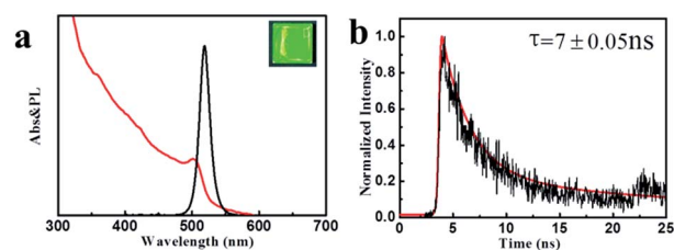
Fig. 3 (a) UV-vis absorption and PL emission spectra (inset: image ( \lambda_{\text{ex}} = 365 nm) \text{CsPbX}_3 NCs). (b) Time-resolved PL decay and fitting curve for the colloidal \text{CsPbBr}_3 NCs sample.
