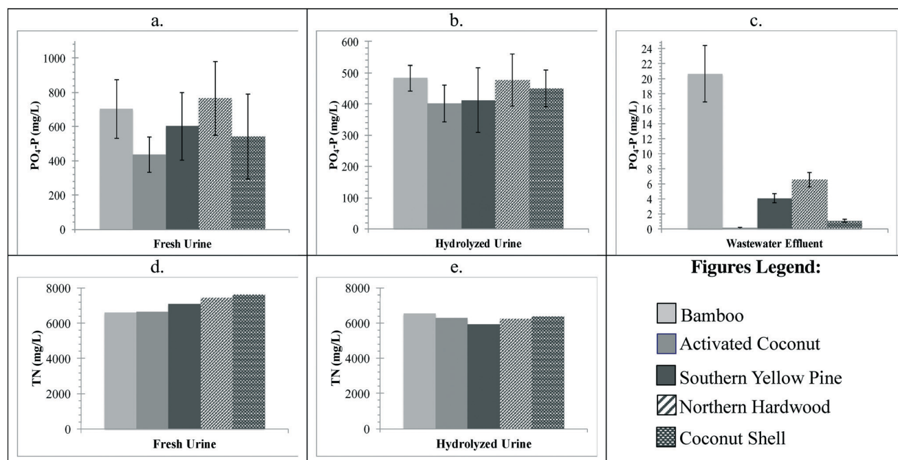
Fig. 3 Phosphate concentrations upon completion of batch tests at 40 g L -1 dose in a. fresh urine ( C_0 = 619 mg L -1 PO 4 -P), b. hydrolyzed urine ( C_0 = 438 mg L -1 PO 4 -P), and c. wastewater effluent ( C_0 = 1.54 mg L -1 PO 4 -P). Error bars indicate one standard deviation from seven sets of triplicate samples. Nitrogen removal by biochar for representative batches in d. fresh urine ( C_0 = 7362 mg L -1 TN) and e. hydrolyzed urine ( C_0 = 7092 mg L -1 TN).
