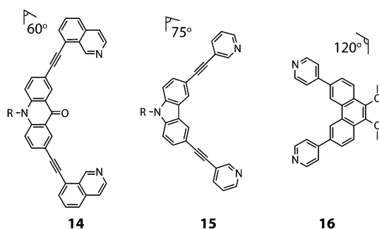
Fig. 9 The angularly distinct bis-monodentate ligands ( 14 – 16 ) used to assemble [\text{Pd}_2\text{L}^{\text{A}}_n\text{L}^{\text{B}}_{4-n}]^{4+} heteroleptic cages ( R = \text{C}_6\text{H}_{13} ).
