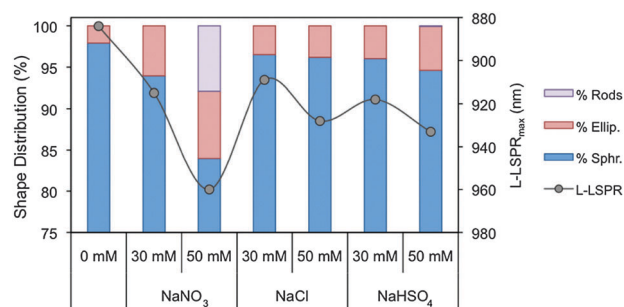
Fig. 7 Micelle shape distribution (spherical, ellipsoidal and rod-like micelles) in growth solutions at different Hofmeister salt concentrations and the \text{L-LSPR}_{\text{max}} of the rods grown in those solutions.
