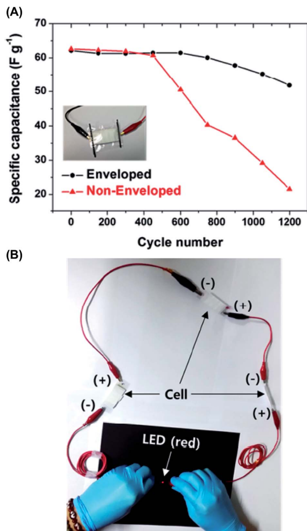
Fig. 7 (A) Long-term cycling stability test profile of enveloped and non-enveloped NaCl-AGAR SCs performed at a scan rate of 100 mV s -1 and (B) digital image of an LED activated by the NaCl-AGAR SC. Reprinted with permission from ref. 46. Copyright © 2015 American Chemical Society.
