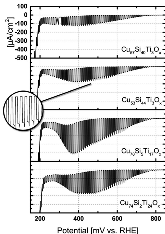
Fig. 5 Linear sweep PEC voltammograms of four selected measurement areas. Cu-rich (Cu >70 at%) samples from the Cu–Ti–O sub-system show highest photocurrent densities but also highest dark/corrosion currents. The photocurrents of the measurement areas close to \text{Cu}_{50}\text{Ti}_{50}\text{O}_x show significantly lower photocurrent densities but also lower dark currents. All samples have the same photocurrent onset potential at around 0.8 V vs. RHE. At around 0.2 V vs. RHE the rapid increase of the dark current indicates gas evolution.
