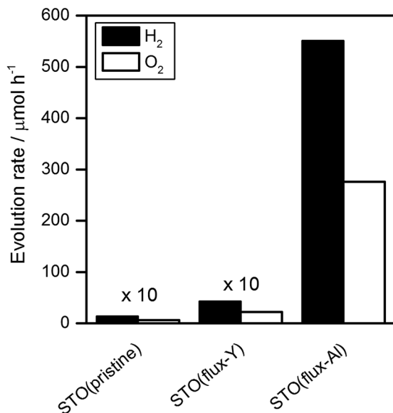
Fig. 3 Water splitting activity of \text{SrTiO}_3 photocatalysts. Reaction conditions: catalyst, 0.1 g; cocatalyst, \text{Rh}_{2-y}\text{Cr}_y\text{O}_3 (Rh 0.1 wt%, Cr 0.1 wt%); reaction solution, 100 mL \text{H}_2\text{O} ; light source, 300 W Xe lamp ( \lambda > 300 nm).
