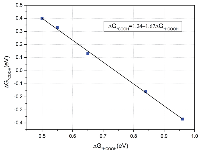
Fig. 9 The relationship between formation free energy of \text{*COOH} and \text{*HCOOH} intermediates.
