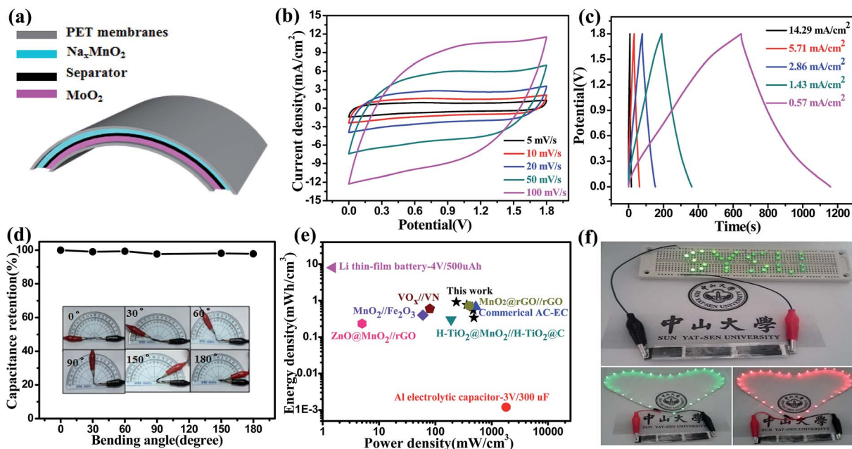
Fig. 5 (a) A schematic illustration of the structure of a flexible \text{Na}_x\text{MnO}_2/\text{CC}/\text{MoO}_2/\text{CC} ASC with two electrodes separated by the TF45 (NKK) membrane (separator); (b) CV curves of the ASC at different scan rates; (c) GCD curves of the ASC at different current densities; (d) stability performance of the ASC collected at different bending angles (the inset shows the flexibility under the different bending angles); (e) Ragone plots of the \text{Na}_x\text{MnO}_2/\text{CC}/\text{MoO}_2/\text{CC} ASC device. The values reported in the literature for other ASC devices are added for comparison; (f) a SYSU logo consisting of 32 green LEDs and a piece of green LED soft rope light powered by the assembled ASCs with three in series.
