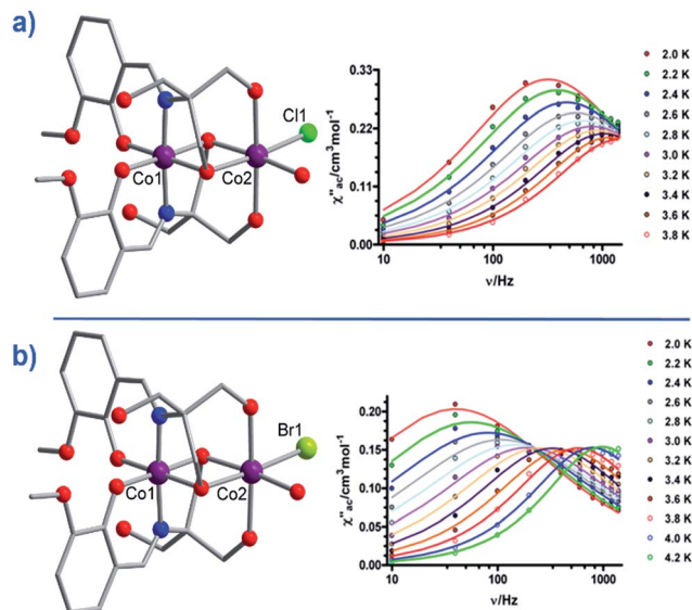
Fig. 15 Molecular structures of [\text{Co}^{\text{III}}\text{Co}^{\text{II}}(\text{LH}_2)_2(\text{X})(\text{H}_2\text{O})](\text{H}_2\text{O})_4 and the frequency dependence of the out-of-phase magnetic susceptibility collected in a 1000 Oe dc field. (a) \text{X} = \text{Cl} (21) and (b) \text{X} = \text{Br} (22). Colour code: purple (Co), bright green (Cl), light green (Br), blue (N), red (O), grey (C). Hydrogen atoms omitted for clarity. Reprinted with permission from ref. 44. Copyright (2014) American Chemical Society.
