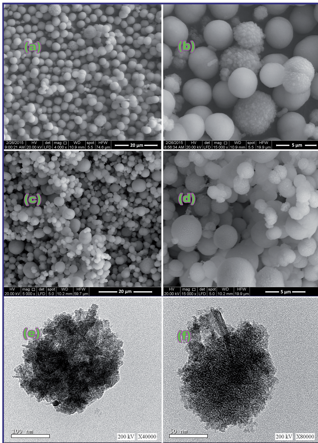
Fig. 4 FE-SEM images of the as-synthesized CoCO 3 /FeCO 3 nanocomposite (a and b) and CoFe 2 O 4 product (S46_600 (c and d)); low and high magnification TEM images of CoCO 3 /FeCO 3 nanocomposite (e and f), respectively, where (a and c) are low magnification FE-SEM images, while (b and d) are high magnification FE-SEM images.
