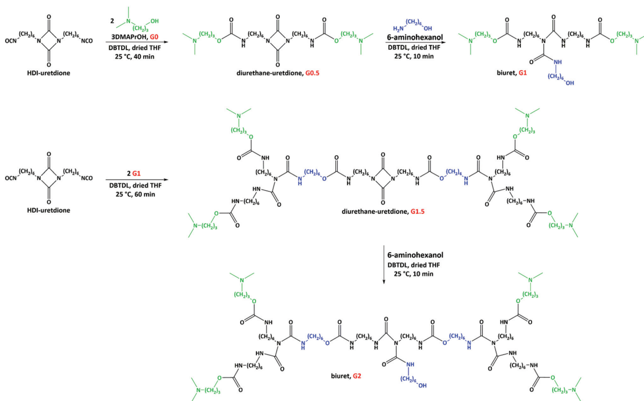
Fig. 1 Reaction pathway for the preparation of the first and second generation of poly(urethane-biuret) dendrons with a hydroxyl focal point. HDI-uretdione: hexamethylene diisocyanate uretdione, 3DMAPrOH: 3-dimethylamino-1-propanol, DBTDL: dibutyltin dilaurate.
