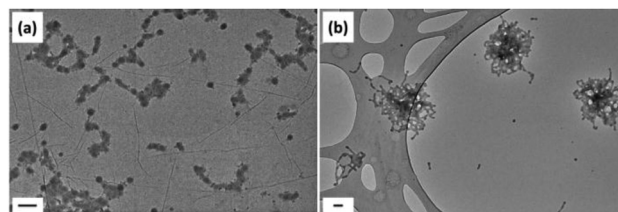
Fig. 4 Representative unstained dry-state TEM images on GO grids of 3-DMSO annealed by different methods: (a) sample was heated at 60 °C for 45 min and then cooled down in an oil bath; (b) sample was heated from 15 °C to 60 °C and then cooled down from 60 °C to 15 °C at a rate of 1 °C min -1 and repeated 3 times in total. Scale bar: 100 nm.
