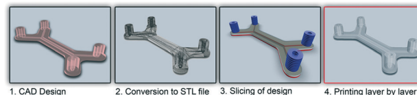
Fig. 1 The additive manufacturing process. The CAD file is converted into a standard triangulation language (STL) file. The STL file is digitally sliced into individual layers that are sequentially realised to build an object in a layer-by-layer manner.
