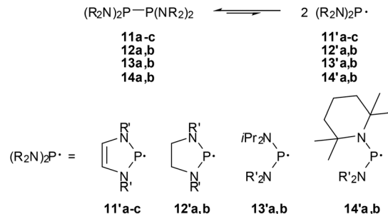
Scheme 13 P–P bond dissociation equilibria for tetraamino-diphosphines (R' = t Bu ( 11a ), 2,6-Me 2 C 6 H 3 ( 11b ), 2,6-iPr 2 C 6 H 3 ( 11b , 12a ), 2- t Bu 2 C 6 H 4 ( 12b ), i Pr ( 13a , 14b ), SiMe 3 ( 13b ), Et ( 14a )).
