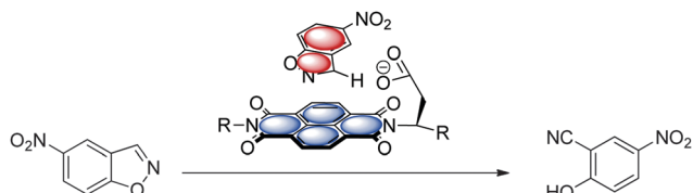
Fig. 37 Schematic representation of the anion– \pi supported Kemp's elimination as reported by Zhao et al. 11a,c
