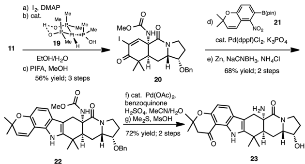
Scheme 3 Synthesis of fused hexacycle 23 . (a) Iodine (3.0 equiv.), DMAP (3.0 equiv.), pyridine/ \text{CCl}_4 , 60 ^\circ\text{C} , 22 h, 77%; (b) 19 (30 mol%), EtOH/ \text{H}_2\text{O} , rt, 4 days, 82%; (c) PIFA (1.1 equiv.), MeOH, 0 ^\circ\text{C} to rt, 16 h, 89%; (d) 21 (1.5 equiv.), dppfPdCl 2 (10 mol%), K 3 PO 4 (3.75 equiv.), DMF, 40 ^\circ\text{C} , 16 h, 94%; (e) Zn (excess), NaCNBH 3 (5.0 equiv.), sat. aq. NH 4 Cl, MeOH, rt, 2 h, 71%; (f) Pd(OAc) 2 (0.40 equiv.), benzoquinone (1.5 equiv.), cat. H 2 SO 4 , MeCN/ \text{H}_2\text{O} , rt, 17 h, 77%; (g) Me 2 S (20 equiv.), MsOH, 40 ^\circ\text{C} , 15 h, 93%. DMAP = 4-dimethylaminopyridine; PIFA = [bis(trifluoroacetoxy)iodo]benzene; dppf = 1,1'-bis(diphenylphosphino)ferrocene; DMF = dimethylformamide; Ms = methanesulfonyl; Bn = benzyl.
