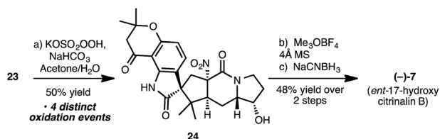
Scheme 4 Completion of the synthesis of 17-hydroxy-citrinalin B ( 7 ). (a) Oxone® (11.4 equiv.), NaHCO 3 , acetone/ \text{H}_2\text{O} , 0 ^\circ\text{C} to rt, 2 h, 50%; (b) Me 3 OBf 4 (12 equiv.), CH 2 Cl 2 , 4 Å MS, 45 ^\circ\text{C} , 16 h, then NaCNBH 3 (excess), MeOH, 0 ^\circ\text{C} , 30 min, 48%. Oxone® = potassium peroxomonosulfate; MS = molecular sieves.
