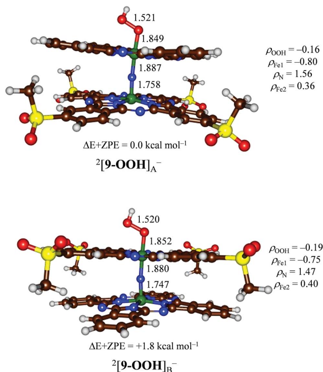
Fig. 7 DFT optimized geometries of 2[\text{9}-\text{OOH}] at the B3LYP level of theory. Bond lengths are in angstroms and spin densities ( \rho ) in atomic units.
