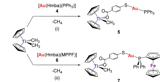
Scheme 1 Preparation of heterometallic titanocene-gold complexes [(\eta\text{-C}_5\text{H}_5)_2\text{Ti}(\text{CH}_3)(\text{OC}(\text{O})\text{C}_6\text{H}_4\text{SAu}(\text{PR}'_2))] ( \text{R} = \text{R}' = \text{Ph} , 5 ; \text{R} = \text{Ph} , \text{R}' = \text{ferrocene} , 7 ). (i) THF/toluene 1.5 : 1, RT, 1 h; (ii) acetonitrile/toluene 3 : 1, RT, 1 h.
