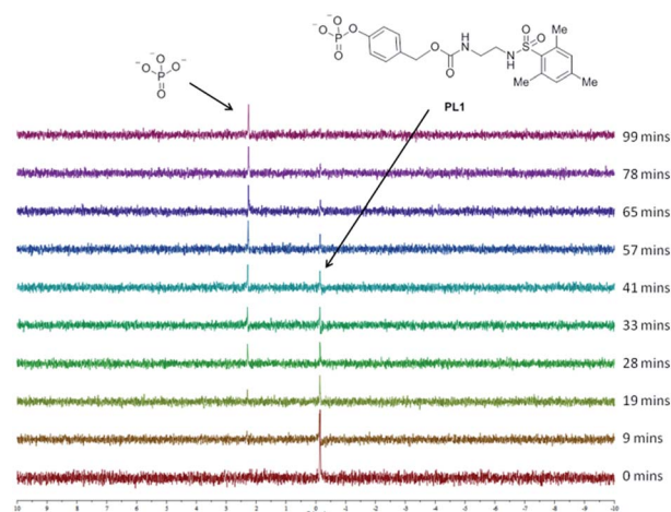
Fig. 3 Stacked 31 P NMR plots of PL1 after addition of ALP.
