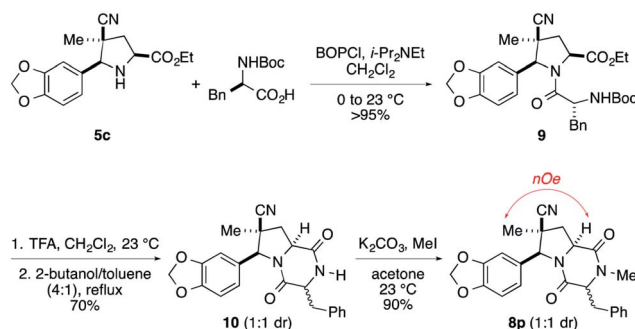
Scheme 2 An alternate route to dioxopiperazine intermediates.
