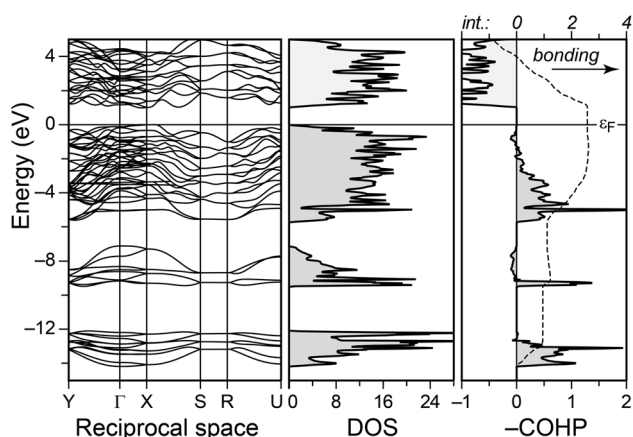
Fig. 2 TB-LMTO-ASA electronic band structure and densities of states (DOS) for \text{Sb}_2\text{Se}_3 , and exemplary crystal orbital Hamiltonian population (COHP) curve for the short Sb(2)–Se(1) contact. The energy integral (“int.”) is given by a dashed line. Negative expectation values of the Hamiltonian reflect stabilisation, and thus we plot -\text{COHP} as is convention. 30c The Fermi level \epsilon_F is set as the energy zero.
