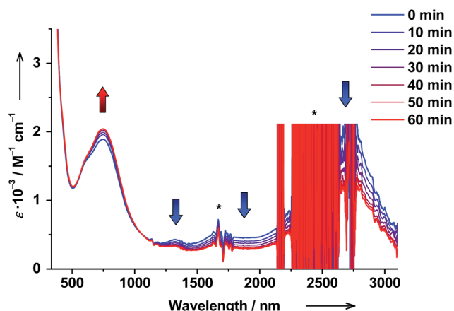
Fig. 10 Changes in absorption spectrum of trans -6 dissolved in toluene upon UV irradiation at RT ( c = 3.7 \times 10^{-4} M, \lambda = 320 \pm 8 nm, 1000 W Xe lamp). Signals marked with asterisk (*) are due to solvent or change of detector.
