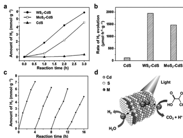
Fig. 17 Photocatalytic activity of MS_2 - CdS nanohybrids for hydrogen evolution reaction. (a) Time-dependent photocatalytic H_2 evolution for WS_2 - CdS , MoS_2 - CdS and pure CdS ; (b) comparison of the H_2 evolution rate under visible light irradiation for WS_2 - CdS , MoS_2 - CdS and pure CdS ; (c) cycling test of photocatalytic H_2 evolution for WS_2 - CdS ; (d) schematic illustration of the photocatalytic process of MS_2 - CdS nanohybrids in lactic acid solution (reproduced with permission from ref. 229. Copyright 2015 John Wiley & Sons, Inc.).
