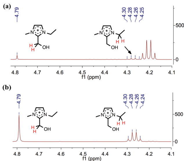
Fig. 6 (a) New ^1\text{H} NMR peaks (4.8–4.1 ppm) observed from the reaction of [\text{C}_2\text{C}_1\text{im}][\text{OAc}] , 1a , with D-(+)-glucose, 12 , after heating at 120 °C for 24 hours, assigned to the [\text{C}_2\text{C}_1(\text{HO})\text{C}_1^2\text{im}]^+ cation. (b) ^1\text{H} NMR spectrum of synthesised [\text{C}_2\text{C}_1(\text{HO})\text{C}_1^2\text{im}][\text{OAc}] , 17 , for comparison.
