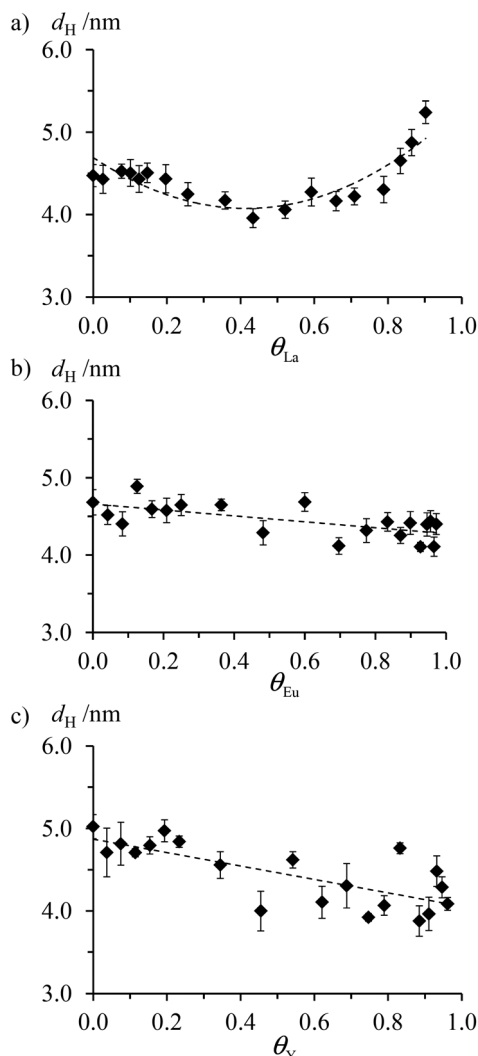
Fig. 7 Hydrodynamic diameters for the lanthanidopolymers [L3^{N=20}(Ln(hfac)_3)_m] as a function of the occupancy factor \theta_{Ln} for lanthanide loadings with (a) [La(hfac)_3]_m , (b) [Eu(hfac)_3]_m and (c) [Y(hfac)_3]_m ( CH_2Cl_2 + 0.15 \text{ mol dm}^{-3} diglyme at 293 K). The trendlines are only guides for the eyes.
