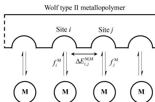
Fig. 1 Thermodynamic model for the successive intermolecular connections of metallic units to a one-dimensional multi-site receptor L possessing N available binding sites. f_i^{\text{M}} and \Delta G_i^{\text{M}} = -RT\ln(f_i^{\text{M}}) are the non-cooperative intrinsic affinity, respectively free energy of connection of site i for the entering metal and \Delta E_{ij}^{\text{M,M}} is the free energy of interaction occurring when two adjacent sites i and j are occupied.
