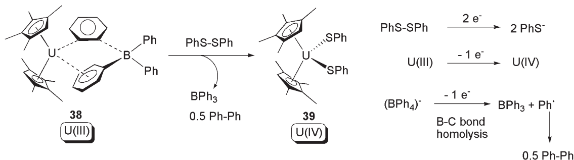
Scheme 24 Oxidative addition of a U(III) compound by PhS-SPh, with the assistance of 1-electron donation from the (BPh 4 ) - ligand. 50
