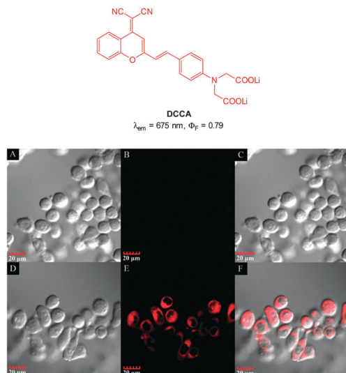
Fig. 41 Top: structure of copper ligand DCCA . Bottom: confocal fluorescence images in KB cells: (A–C) cells incubated with DCCA 2 –Cu(II) alone. (D–F) Cells incubated with DCCA 2 –Cu(II), then \text{K}_4\text{P}_2\text{O}_7 . Emission collected at 630–730 nm, excitation at 405 nm. Bright field (A and D), fluorescence (B and E) and overlap field (C and F). Image reproduced with permission. 192
