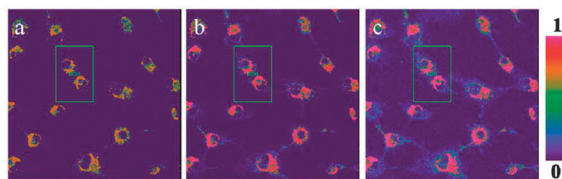
Fig. 52 Top: structure and reaction of HS-Cy with \text{HS}^- . Bottom: confocal fluorescence ratiometric images of endogenous \text{HS}^- in living A549 cells. A549 cells loaded with 5 \text{ mM HS-Cy} for 30 min (a). Cells were pre-stimulated with SNP, then incubated with HS-Cy for 10 min (b) and 20 min (c). Scale = 50 \text{ nm} . Image reproduced with permission. 222
