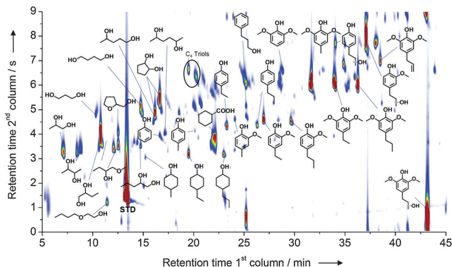
Fig. 7 Speciation of the products obtained from the catalytic biorefining of poplar wood in the presence of RANEY ® Ni at 180^\circ\text{C} for 3 h (2-PrOH/ \text{H}_2\text{O} , 7 : 3, v/v). Reproduced with permission from ref. 35. Copyright 2014, Wiley-VCH Verlag GmbH & Co. KGaA, Weinheim.
