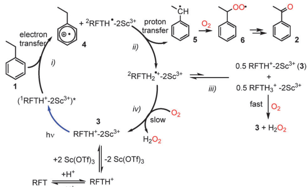
Scheme 3 Proposed mechanism for the photocatalytic aerobic oxidation of ethylbenzene ( 1 ) to acetophenone ( 2 ) with RFT in presence of \text{Sc}^{3+} -ions and HCl.
