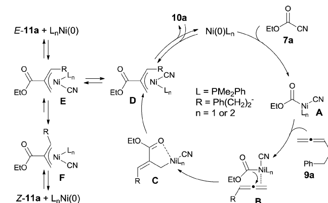
Scheme 8 Proposed mechanism for Ni-catalyzed cyanoesterification on 1,2-diene.
