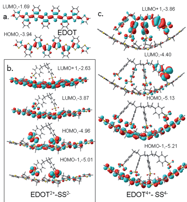
Fig. 6 (a) Nature of HOMO and LUMO in EDOT; (b) nature of HOMO – 1, HOMO, LUMO and LUMO + 1 in \text{EDOT}^{2+}\text{--SS}^{2-} ; (c) nature of HOMO – 1, HOMO, LUMO and LUMO + 1 in \text{EDOT}^{4+}\text{--SS}^{4-} . The red and cyan colors represent different signs of the wave functions in the molecular orbitals. The energies of the orbitals are reported in eV.
